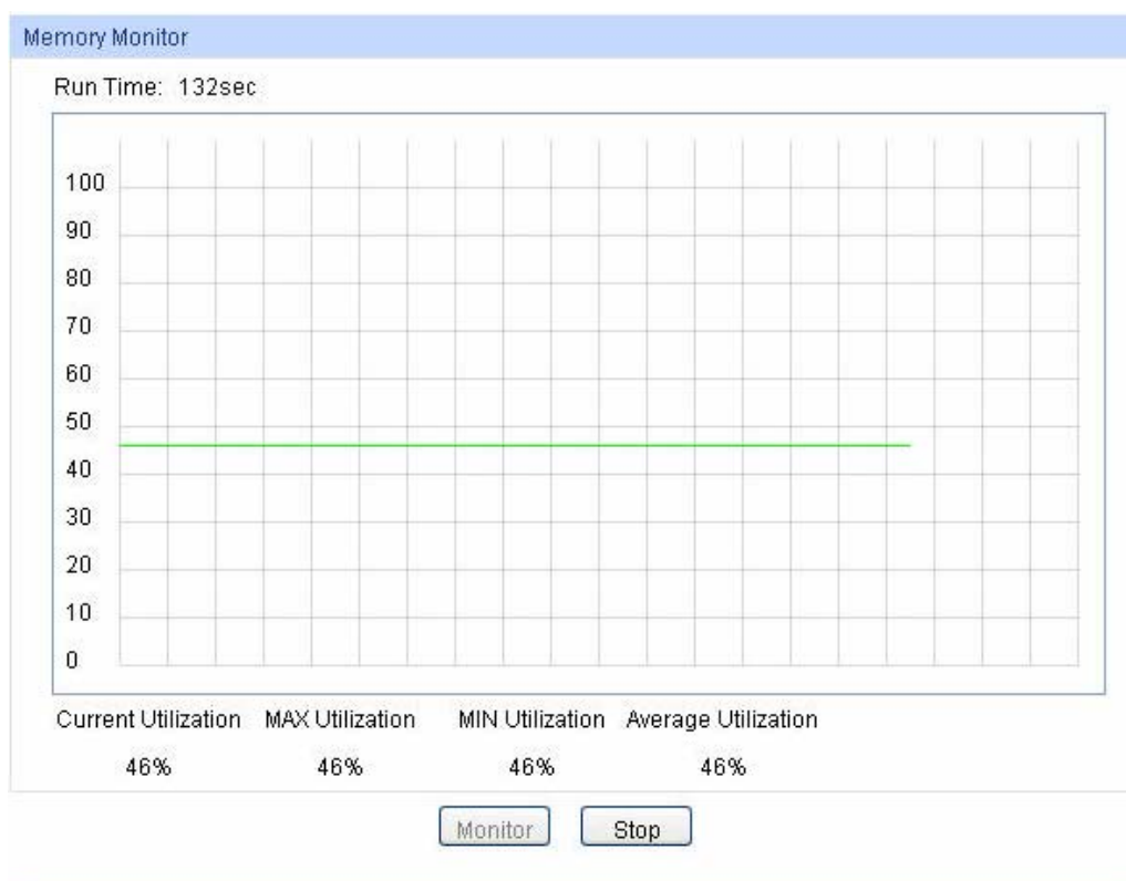
Figure 12-2 Memory Monitor
