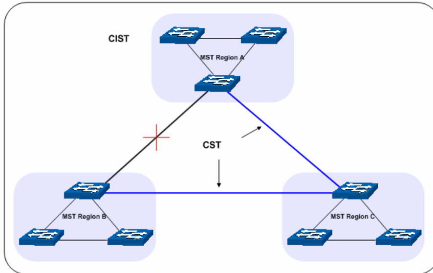
Figure 7-2 Basic MSTP diagram
