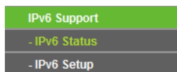
Figure 4-79 IPv6 Support
